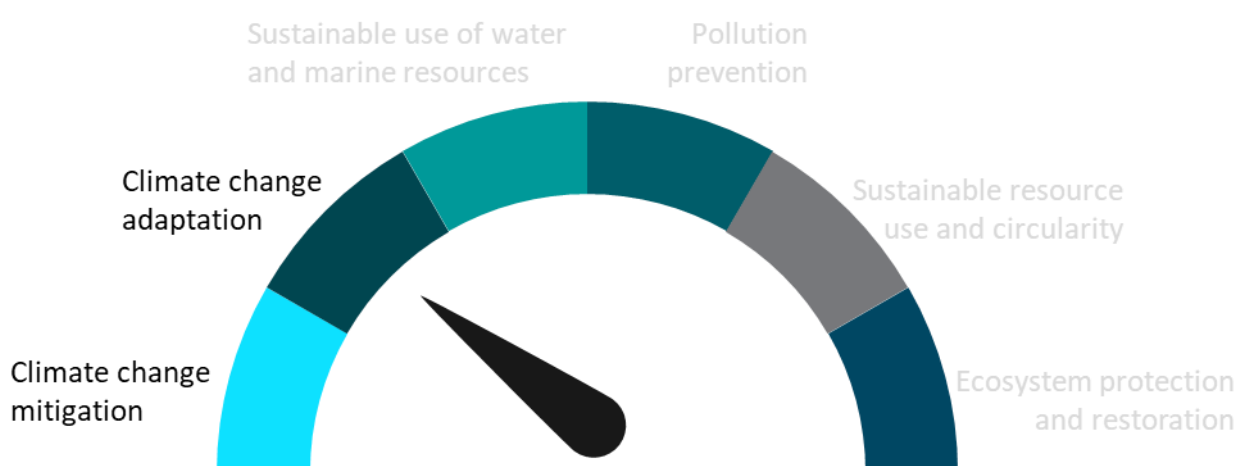
Figure 4: Taxonomy objectives
